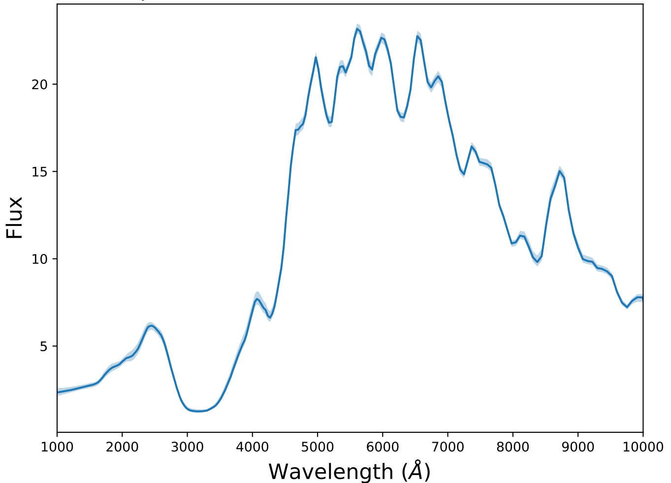
Spectrum 10 for transient CCSN at z=0.40
